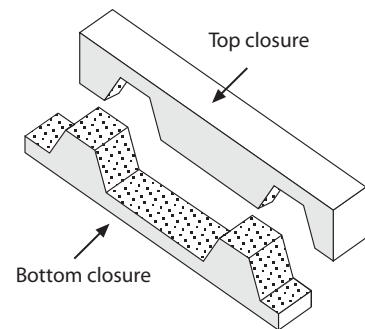
Top & Bottom End Closures (SunSky 12") Figure 22b
