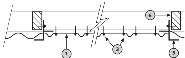
Framed Side Light Horizontal Section
