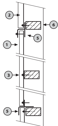
Typical Side Light Vertical Section
