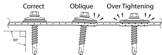
Right & wrong fastener insertion Figure 17
